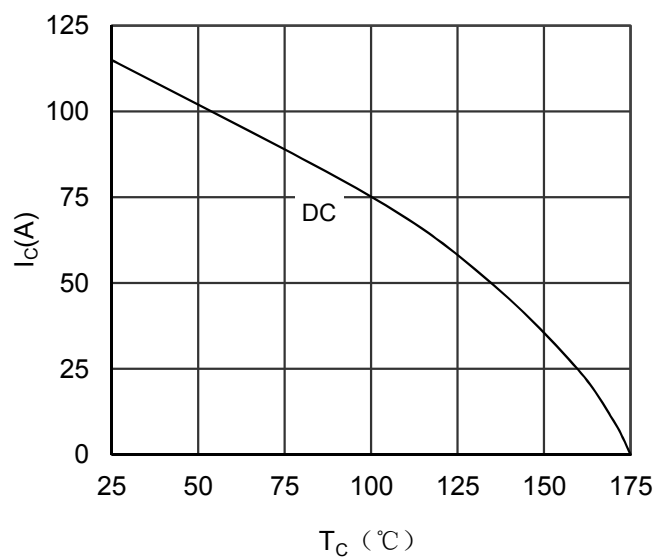
Figure 6. Collector Current vs Case temperature IGBT
